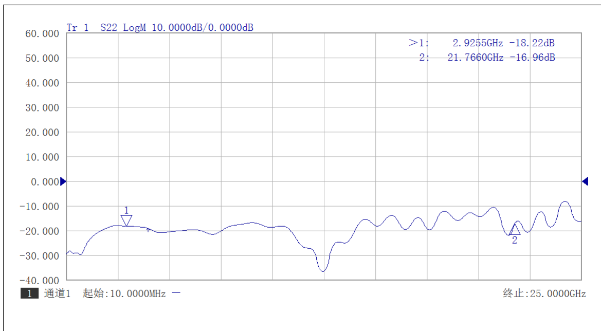
Output Return Loss vs Frequency 10MHz-22GHz
