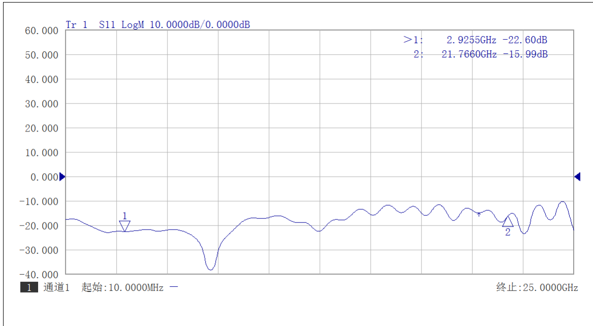
Input Return Loss vs Frequency 10MHz-22GHz
